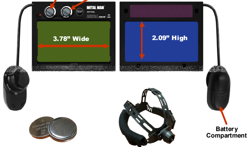
CR2450 Batteries (Included) 6-Point Adjustable Head Gear
